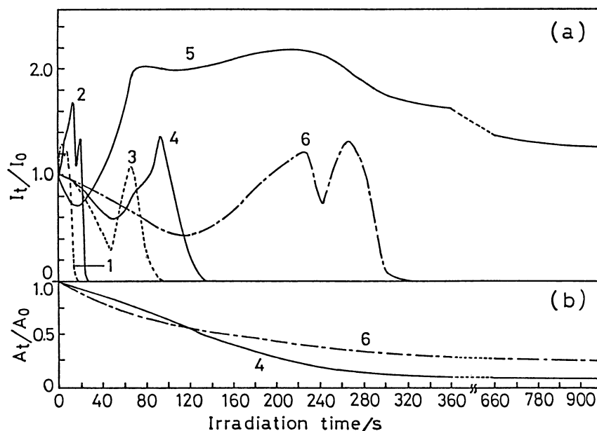
Fig. 1. Read-out intensity change(a) and absorbance change(b) owing to trans \rightarrow cis photoisomerization of azobenzene group in liquid crystals.
