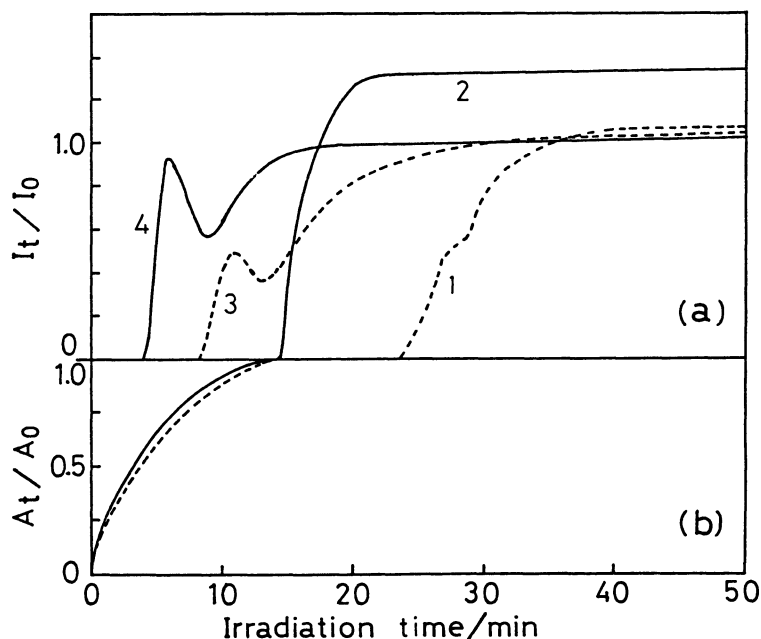
Fig. 2. Reverse phase transition induced by cis \rightarrow trans photoisomerization of II(a) and recovery of absorbance(b).
